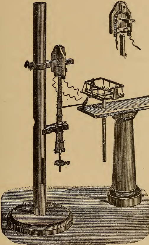
Fig. 16. NEGRO'S FIRST ELECTRO-MOTOR.
